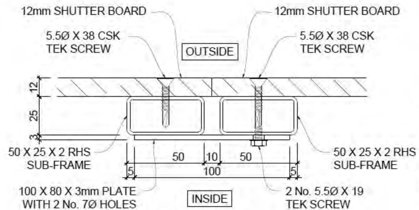
TYPICAL SUBFRAME JOIN DETAIL SCALE 1:2
